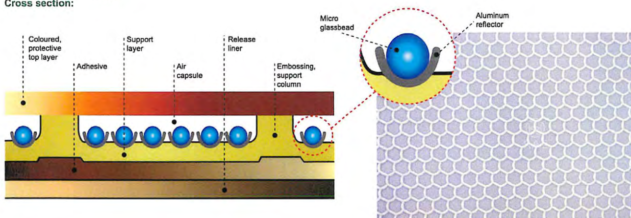
Encapsulated lense type - Cross section:
