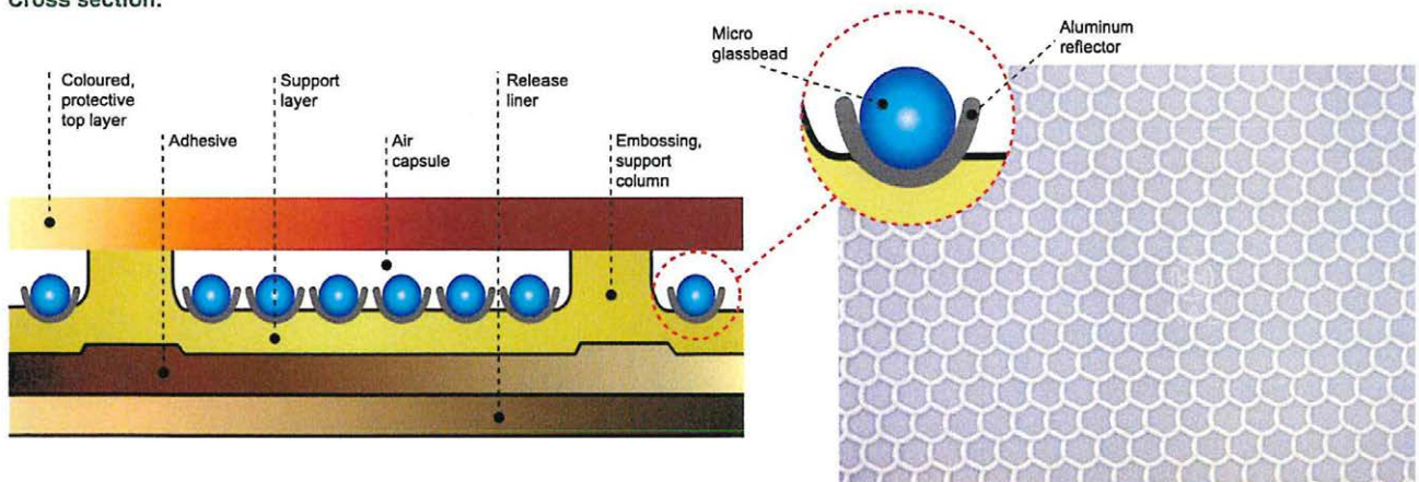
Encapsulated lense type - Cross section:
